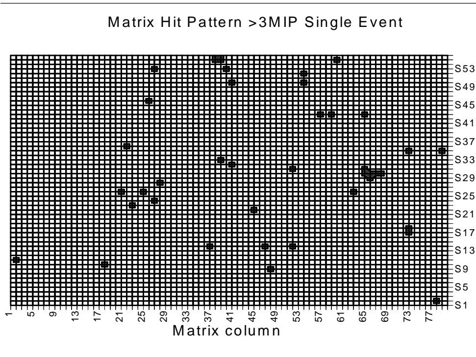
Fig. 3 This figure shows the pattern of hits in the silicon matrix from a single event. Each grid intersection corresponds to a single pixel in the matrix. This event has a deposited energy in the calorimeter of 87 TeV. The hit threshold is 3 MIPs, the typical dividing line between protons and helium.
