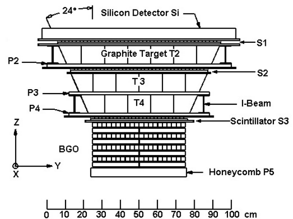
Fig. 1. The ATIC instrument configuration
