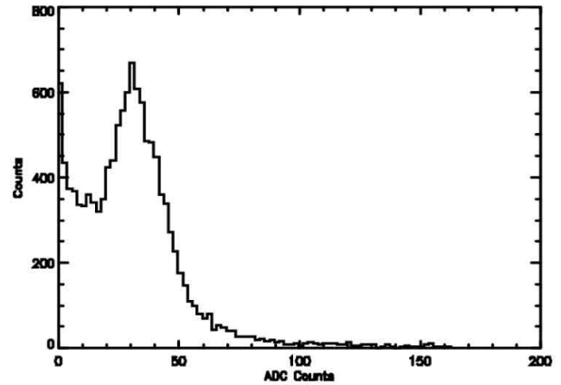
Fig. 3: Pulseheight distribution for cosmic ray muons in low energy range
