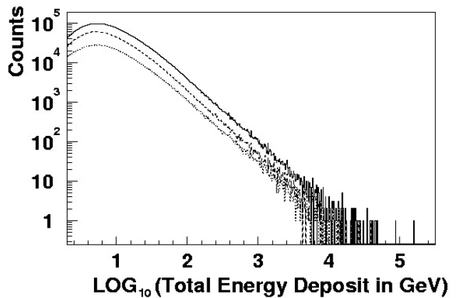
Fig. 4. Particle counts as a function of energy: All particles (solid curve), proton candidates (dashed curve), and helium candidates (dotted curve). No unfolding procedures have been applied.
