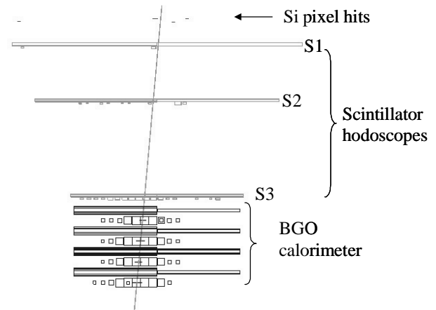
Fig. 1. ATIC detector response to a high energy event ( \sim 5 TeV incident energy) and the reconstructed incident particle trajectory (nearly vertical line) in the ATIC detector system.
