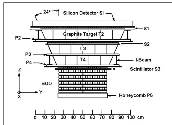
Fig. 1 The ATIC instrument configuration
